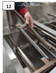
THE BURNER IS REPLACED
