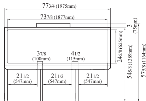
M3R72-3-N-AL TOP VIEW
