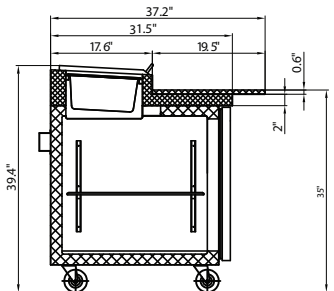
SECTION VIEW
