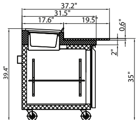
SECTION VIEW
