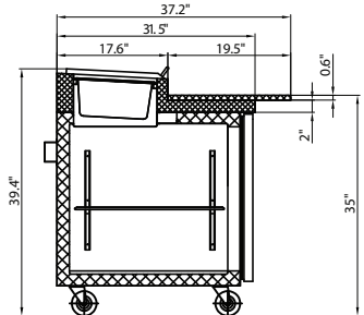
SECTION VIEW
