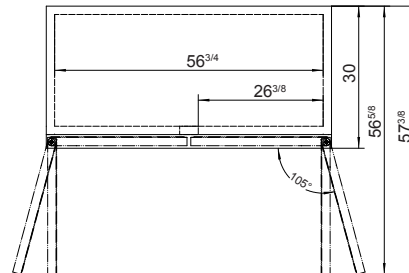
Rear grate
