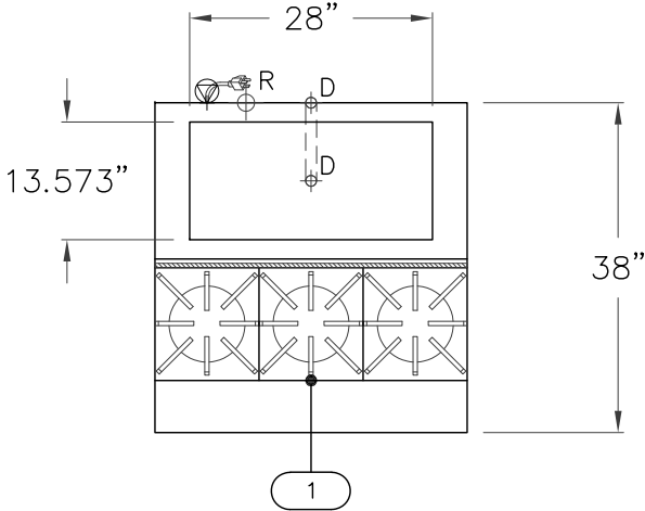
PLAN VIEW WITHOUT PANS BY OTHERS
