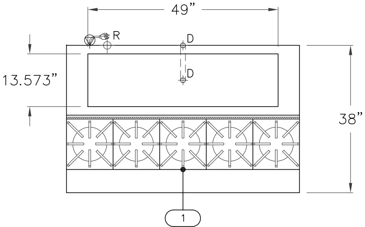
PLAN VIEW WITHOUT PANS BY OTHERS
