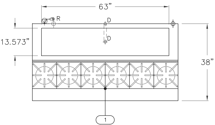
PLAN VIEW WITHOUT PANS BY OTHERS
