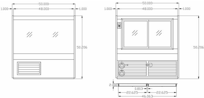
SC-CFS32-6 3 ICE PAN
