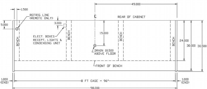
8 FOOT CASE 98"
