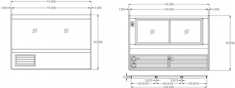
SC-CFS32-8 4 ICE PAN
