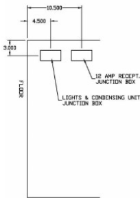
JUNCTION BOX
