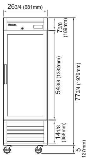
FRONT VIEW
