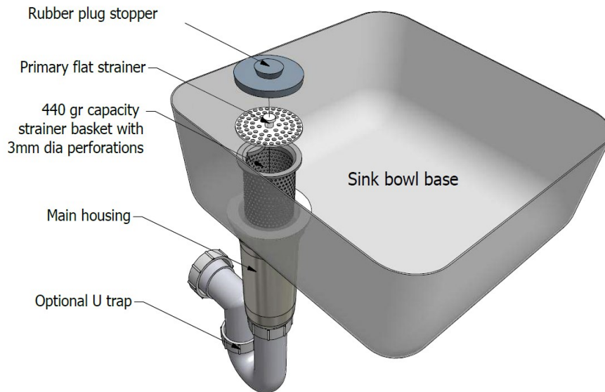
Components Break out View
