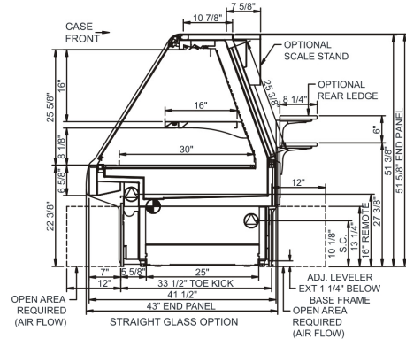
Model Technical Specifications Model L" L1" L2" System Circuit Volts Phs Freq Amps *** Watts Wires NEMA Plug SST Conv. Rack BTUH Para. Rack BTUH Est Wt GMDS4R 48.75 51.00 3.50 Remote(Type I) Circuit #1 110-120 1 60 2.27 234 2+G Leads Multiple 20.00 1296 1200 950 Remote(Type I) Circuit #1 110-120 1 60 2.27 234 2+G Leads Multiple 20.00 1296 1200 Self-Contained Circuit #1 110-120 1 60 10.22 779 2+G 5-15P or L5-15P N/A N/A N/A GMDS5R 60.63 62.88 3.50 Remote(Type I) Circuit #1 110-120 1 60 2.98 288 2+G Leads Multiple 20.00 1728 1600 1,000 Remote(Type I) Circuit #1 110-120 1 60 2.98 288 2+G Leads Multiple 20.00 1728 1600 Self-Contained Circuit #1 110-120 1 60 12.00 1,031 2+G 5-15P or L5-15P N/A N/A N/A GMDS6R 73.13 75.38 3.50 Remote(Type I) Circuit #1 110-120 1 60 3.35 338 2+G Leads Multiple 20.00 2030 1880 1,300 Remote(Type I) Circuit #1 110-120 1 60 3.35 338 2+G Leads Multiple - 2030 1880 Self-Contained Circuit #1 110-120 1 60 14.82 1,071 2+G 5-20P or L5-20P N/A N/A N/A GMDS8R 97.50 99.75 9.00 Remote(Type I) Circuit #1 110-120 1 60 3.84 408 2+G Leads Multiple 20.00 2722 2520 1,600 Remote(Type I) Circuit #1 110-120 1 60 3.84 408 2+G Leads Multiple 20.00 2722 2520 Self-Contained Circuit #1 110-120 1 60 16.00 1,360 2+G 5-20P or L5-20P N/A N/A N/A
