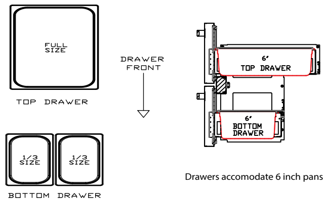
Pan Configuration
