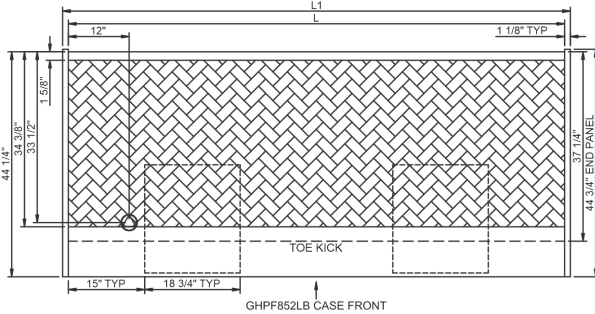
GHPF852LB CASE FRONT
