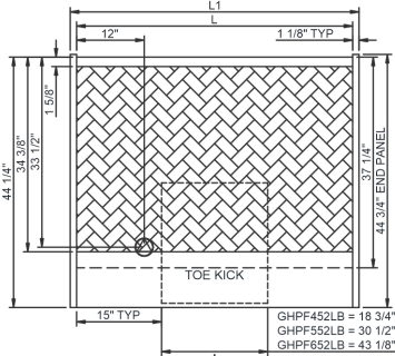
GHPF452LB, GHPF552LB, GHPF652LB CASE FRONT
