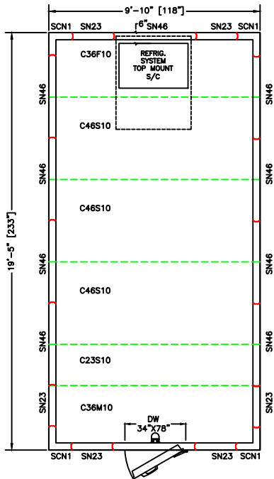
PLAN VIEW RIGHT HINGE SELECT
