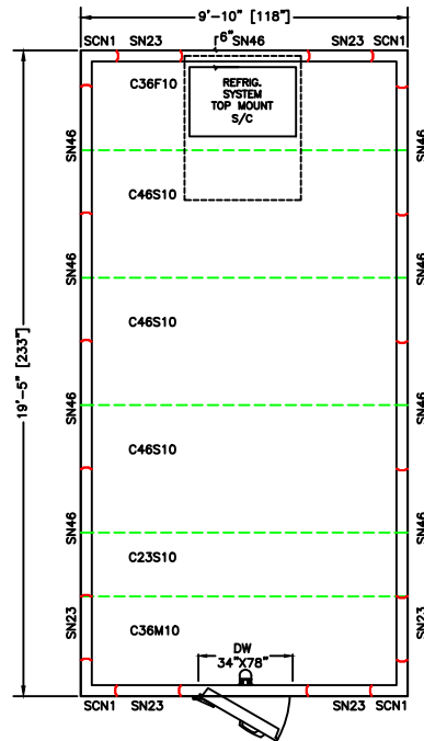
PLAN VIEW LEFT HINGE SELECT
