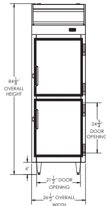
ELEVATION VIEW
