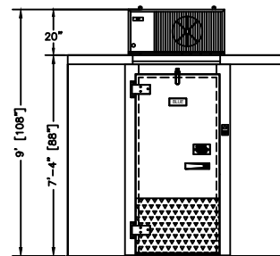
ELEVATION LEFT HINGE
