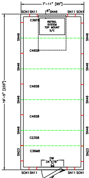
PLAN VIEW RIGHT HINGE SELECT
