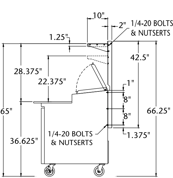
SINGLE SHELF SIDE VIEW
