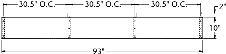
PLAN VIEW NLPT93
