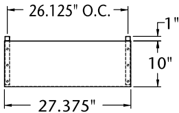
PLAN VIEW NLSP27-8A, NLSMP27-12A
