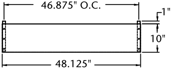
PLAN VIEW NLUR/NLUF48A
