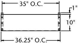
PLAN VIEW NLUR/NLUF36A
