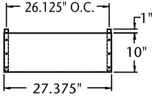
PLAN VIEW NLUR/NLUF27A
