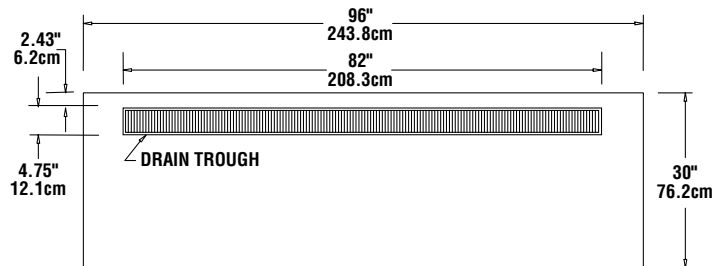
PLAN VIEW KCU-96/ KCU-96-NU
