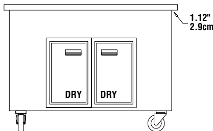
ELEVATION VIEW ALL KCU-50/KCU-74 MODELS (KCU-96 two 36" compartments not shown)
