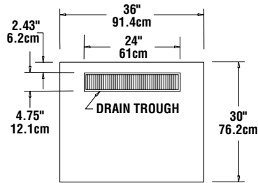
PLAN VIEW KCU-36/ KCU-36-NU
