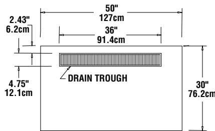
PLAN VIEW KCU-50/ KCU-50-NU
