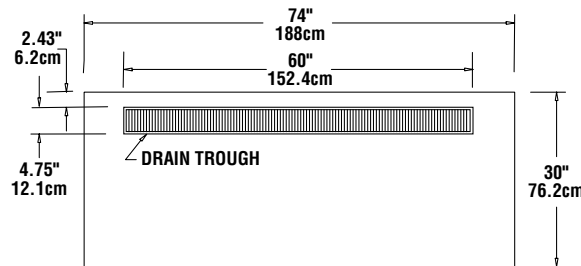
PLAN VIEW KCU-74/ KCU-74-NU
