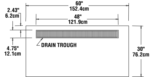
PLAN VIEW KCU-60/ KCU-60-NU
