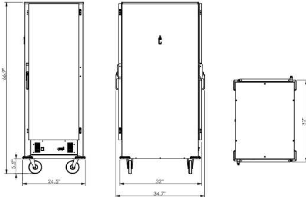
Top View
