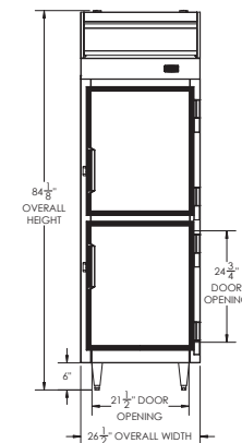
ELEVATION VIEW
