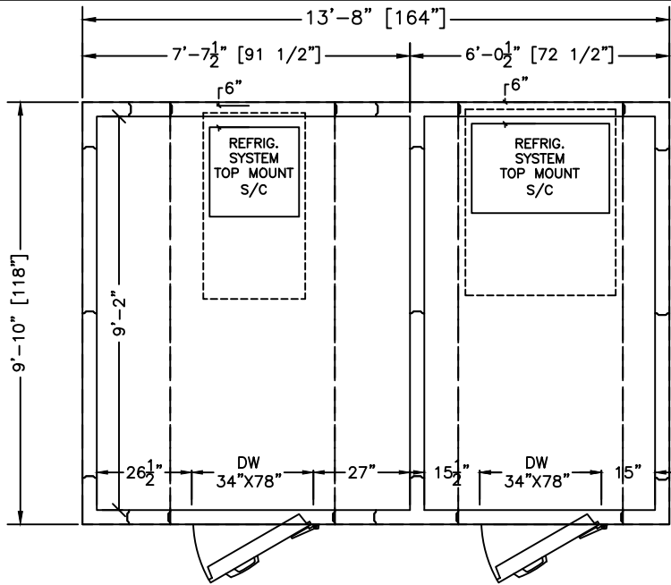
COOLER (WITH FLOOR PANELS)
