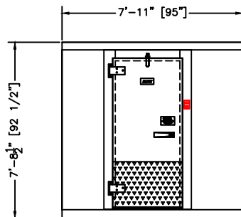
ELEVATION LEFT HINGE
