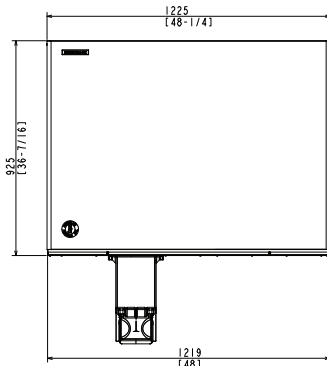
WATER-COOLED
