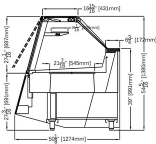
METRO 2 - 54 5/16"H
