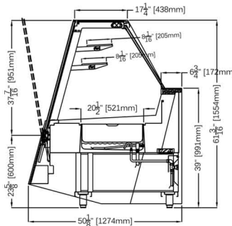
METRO 3 - 61 3/16"H
