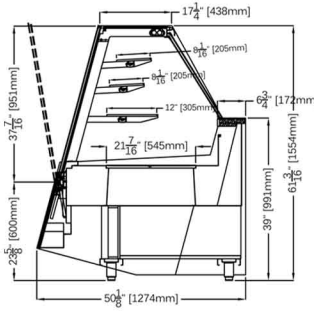
METRO 3 - 61 3/16"H
