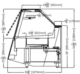
METRO 2 - 54 5/16"H
