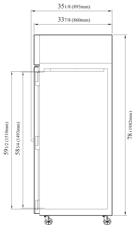
SIDE VIEW
