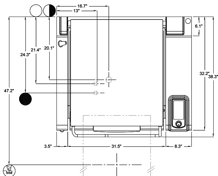
Overhead View (VPP28E)
