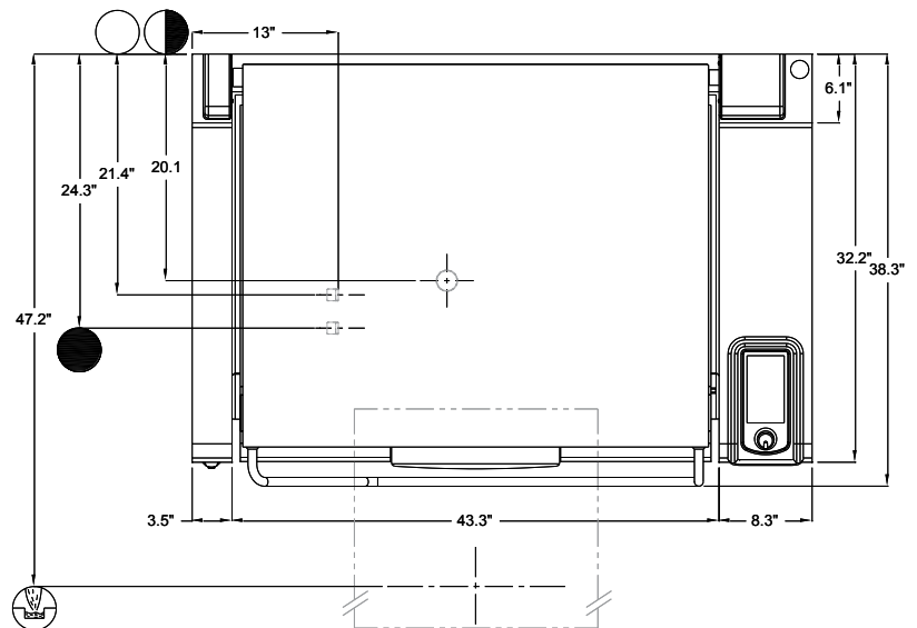
Front View (VPP40E)
