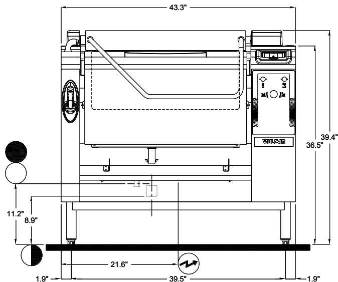
Front View (VPP28E)
