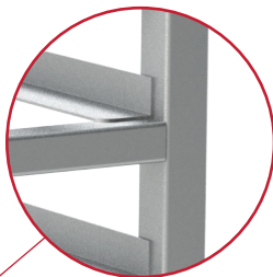
HD Uprights & Cross Braces All welded 1-1/4" square tubular frame with 1" cross braces with all rounded-edges
