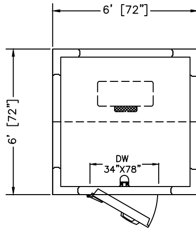
PLAN VIEW LEFT HINGE SELECT
