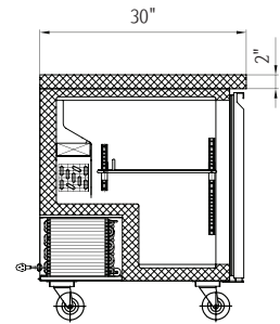
Side Section
