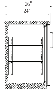
Side Section
