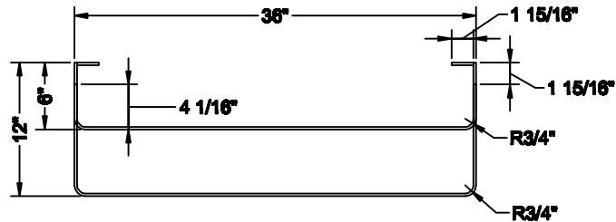
PLAN VIEW
