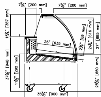
RIGHT VIEW
