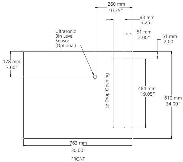
30" Prodigy Plus plan view
