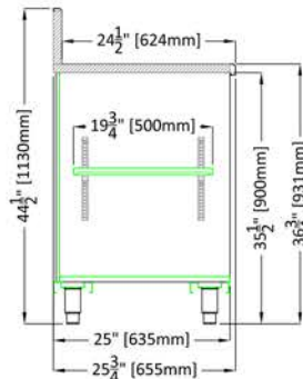
B - 25 3/4"D (655mm) SIDE VIEW
