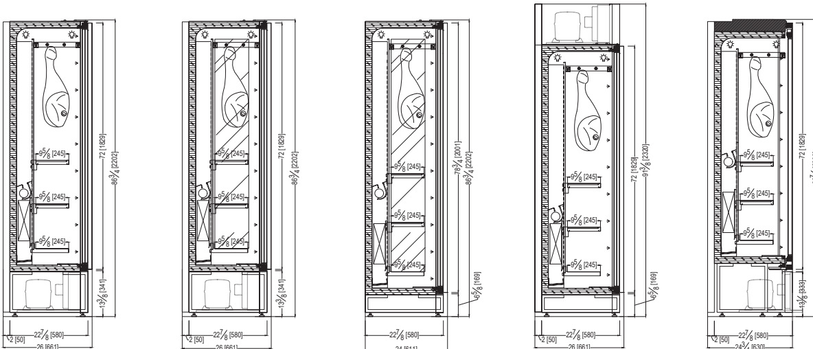
OPTIONAL: SLIDING DOORS ONLY IN SOLID SIDES AND 2100, 2800 MODELS
