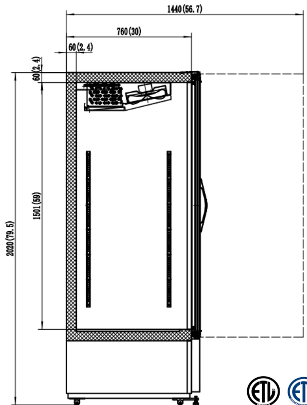
SIDE VIEW
