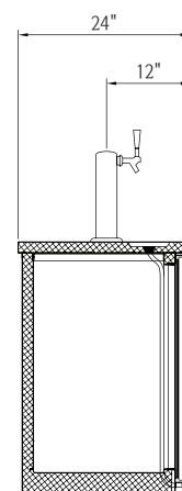
Side Section
