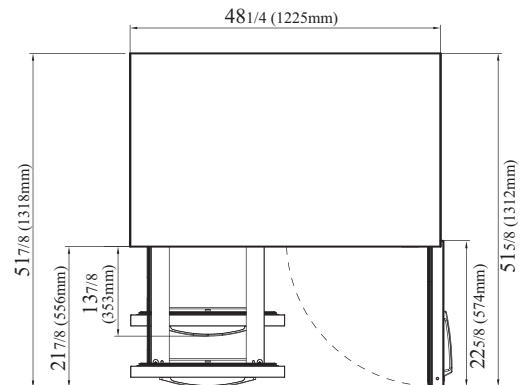
PUR-48-D2R-FB-N TOP VIEW
