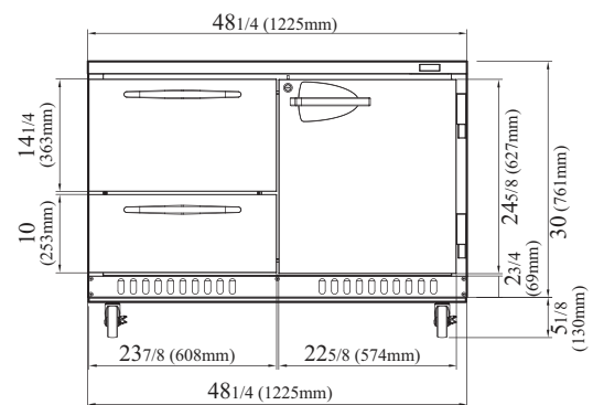
PUR-48-D2R-FB-N FRONT VIEW
