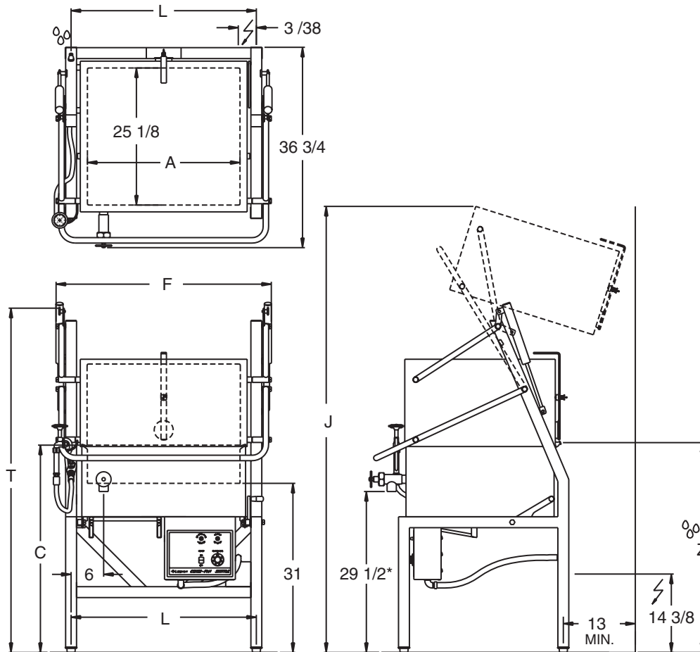
SKITTLE® DIMENSIONS
