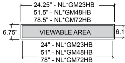
GRAPHIC PANEL DIMENSIONS
