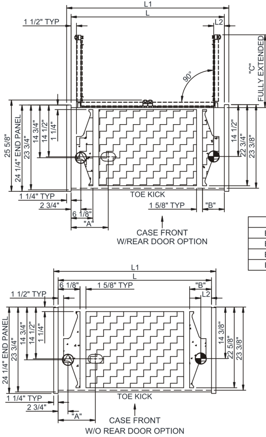
PLAN VIEW
