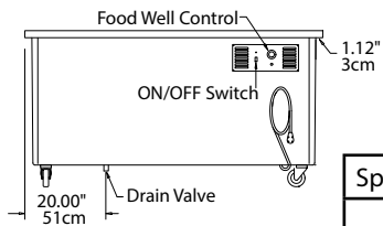
Typical Elevation View All Models
