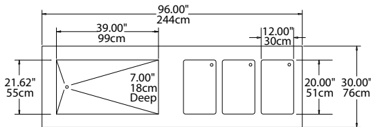
Plan View KH3C-96-NU
