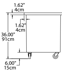
Right End View All Models
