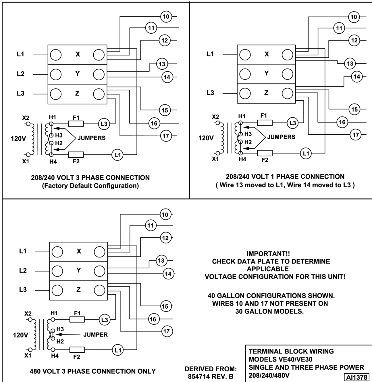
Terminal Block Wiring
