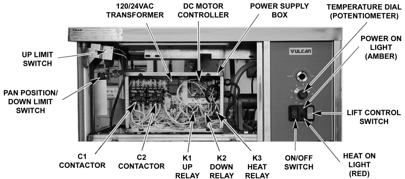
VE30 WITH MOTORIZED LIFT OPTION FRONT VIEW SHOWN
