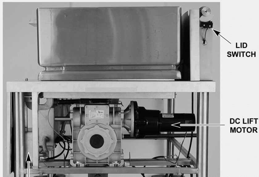
VE30 WITH MOTORIZED LIFT OPTION RIGHT SIDE VIEW SHOWN
