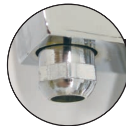
Outlet Tip with Adjustable Water Flow 0.5 - 2.3 GPM @ 60 psi
