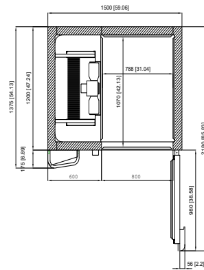
PLAN VIEW
