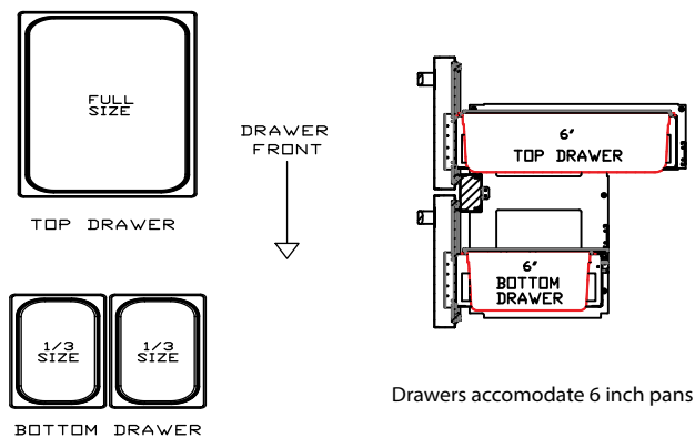
Pan Configuration
