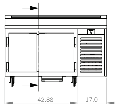
Elevation View
