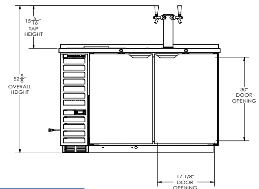
ELEVATION VIEW
