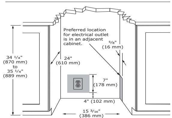
Cabinet Cut-Out
