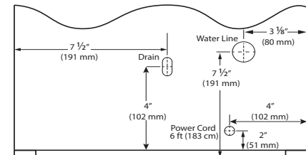
Cabinet Cut-Out
